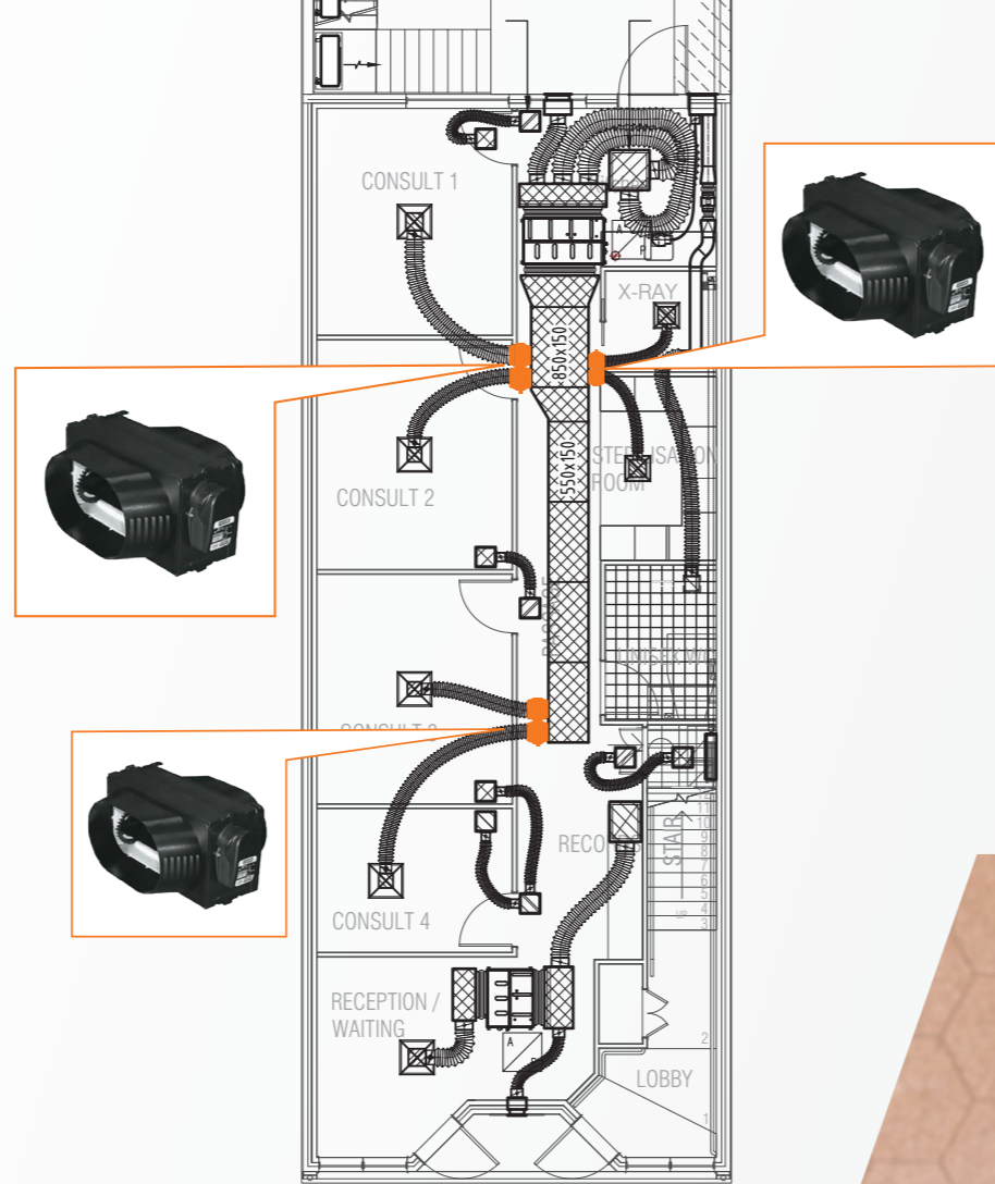
Above: Typical Commercial Air Conditioning Application
